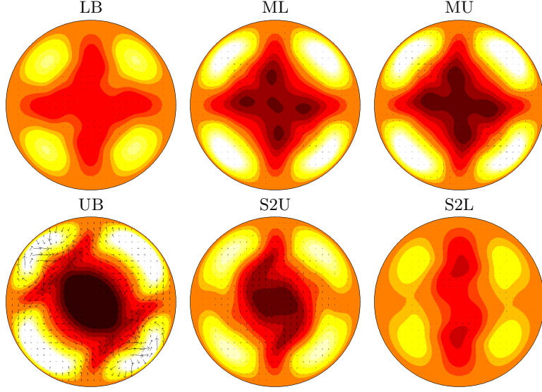
FIGURE 7. Travelling waves for the cell (2.4), reduced to equilibria by the method of slices. Colour map of stream-wise velocity relative to the laminar flow, lighter (darker) indicating positive (negative) w in the range [-0.6, 0.7] . The N2 states (LB, ML, MU and UB) have symmetries (S, Z_2) , where the symmetry C_{2,\theta} is implied. The S2 states originate from a symmetry-breaking bifurcation off the N2 branch and have symmetries S and C_{2,\theta} only. Shown is one fixed pipe section for each of the solutions. As the choice of the stream-wise position of such section is arbitrary, only meaningful comparison of different solutions is by their distance in the symmetry-reduced state space.
