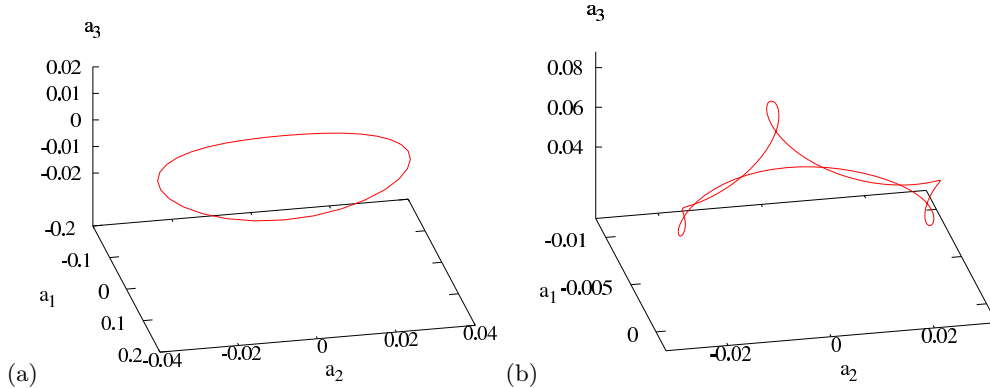
FIGURE 3. Projections of group orbits of two states a (in \approx 100,000 -dimensional state space) onto stationary Frenet-Serret frames given by unit vectors in the directions \{\mathbf{t}_z(a'), \mathbf{t}_\theta(a'), \mathbf{n}_z(a')\} , see (2.15). The state in (a) is a very smooth state, the ‘lower-branch’ travelling wave LB, whereas in (b) it is a snapshot from a turbulent run. The group orbits are generated by all possible axial shifts g(0, \ell)a , and plotted relative to a template point a' . In (a) the state a = a' = a_{\text{LB}}(0) belongs to the “lower-branch” travelling wave \mathcal{M}_{\text{LB}} described in §5.1; in (b) a is a ‘typical’ turbulent state snapshot with its group orbit as seen from the template a' = a_{\text{ML}} . Group orbits are only topologically circles; for strongly nonlinear, turbulent states many Fourier modes are of comparable magnitude, with their sums resulting in highly convoluted group orbits such as (b).
