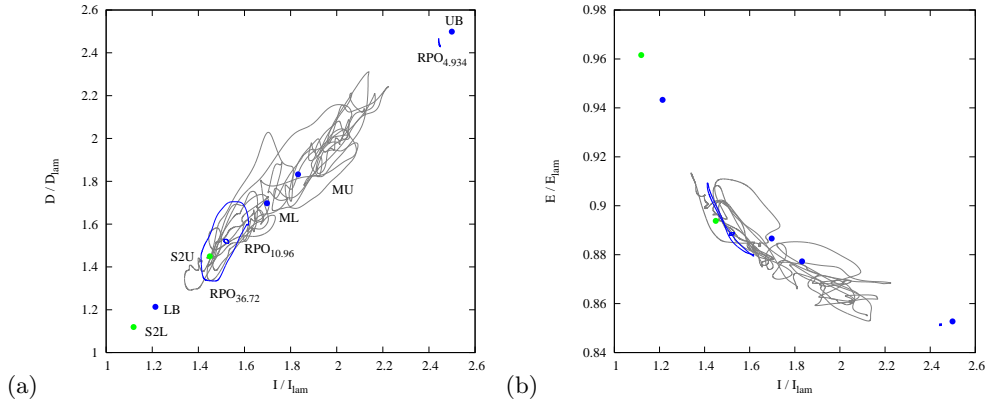
FIGURE 11. Rate of the energy input at the walls I versus (a) the dissipation rate D , and (b) the energy E , see (2.7). Plotted are all invariant solutions of table 1, together with a typical turbulent orbit. The tiny RPO 4.934 is visible as a little twiddle just below UB travelling wave. On the scale of these plots, the Duguet et al. (2008) relative periodic orbit would be indistinguishable from its mother travelling wave.
