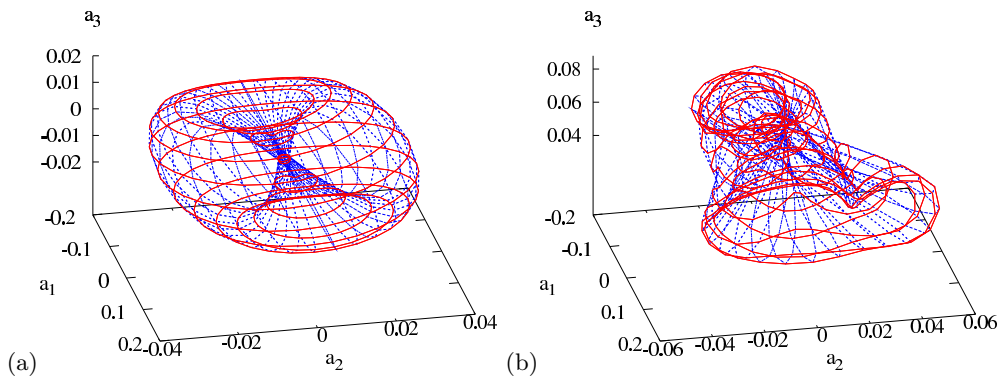
FIGURE 4. As figure 3, but with the full 2-dimensional \text{SO}(2)_\theta \times \text{SO}(2)_z group orbits traced out by shifts in both z and \theta . Loops in solid red correspond to shifts in z , dashed blue loops to shifts in \theta .
