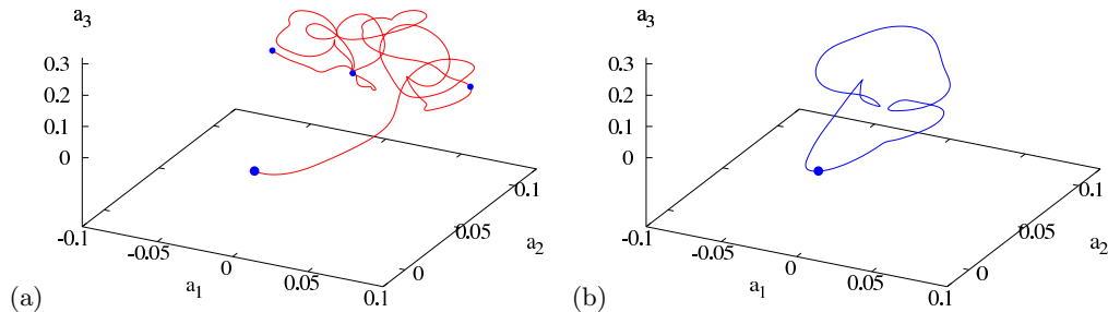
FIGURE 1. Symmetry reduction replaces each full state space trajectory a(t) by a simpler reduced state space trajectory \hat{a}(t) , with continuous group induced drifts quotiented out. Here this is illustrated by the relative periodic orbit \text{RPO}_{36.72} (see figure 9 b) (a) traced in the full state space for three T = 36.72 periods, in the frame moving with the constant axial phase velocity \bar{c} = 1.274 , the average phase velocity of structures estimated from a long simulation; dots are spaced T apart in time; (b) restricted to the symmetry-reduced state space. Both are projected onto the 3-dimensional frame (2.16). In the full state space a relative periodic orbit traces out quasi-periodically a highly contorted 2-torus; in the reduced state space it closes a periodic orbit in one period T .
