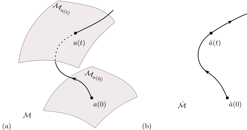
FIGURE 2. (a) The group orbit \mathcal{M}_{a(0)} of state space point a(0) , and the group orbit \mathcal{M}_{a(t)} reached by the trajectory a(t) time t later. (b) Symmetry reduction \mathcal{M} \rightarrow \hat{\mathcal{M}} replaces each full state space group orbit \mathcal{M}_a \subset \mathcal{M} by a single point in the reduced state space \hat{a} \in \hat{\mathcal{M}} .
