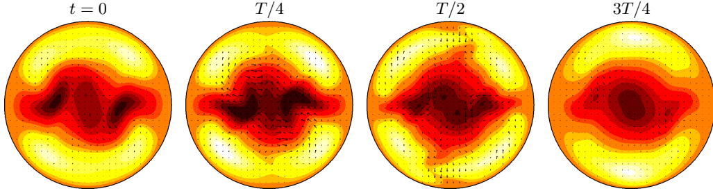
FIGURE 12. Four snapshots of relative periodic orbit RPO_{36.72} at the same fixed pipe section as in (7), reduced by the method of slices into a periodic orbit solution (see movie online ). A colormap of stream-wise velocity is shown, with white (black) indicating positive w = 0.6U (negative w = -0.7U ) velocity with respect to laminar flow. The t = 0 state has been chosen to be the closest passage (in the energy norm) to travelling wave S2U, see (7).
