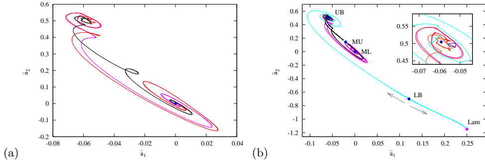
FIGURE 8. (a) Projection of the dynamics local to the ML travelling wave which has been reduced to the equilibrium at (0,0) within the slice. The local spiral of unstable trajectories is now clearly revealed, the ML state having only a single complex unstable eigenvalue within its (S, Z_2) symmetry subspace. (b) All N2 equilibria, perturbations restricted to the (S, Z_2) symmetry subspace. The inset shows an expanded view near the UB state. The dark blue loop is a tiny relative periodic orbit with period T = 4.934 . Axes as in (5.1).
