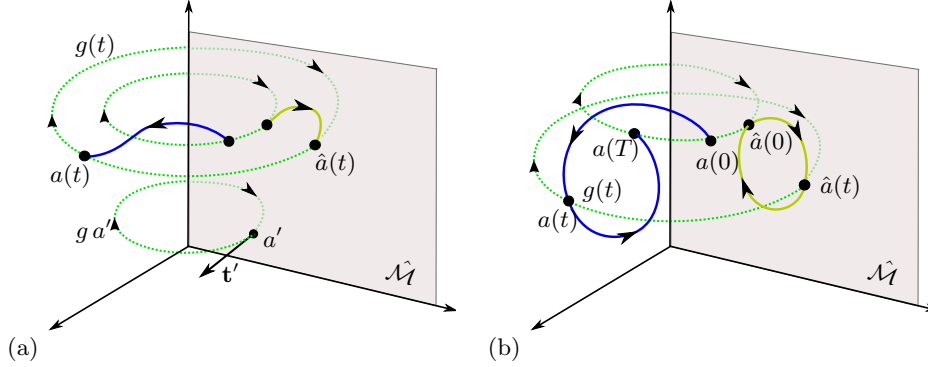
FIGURE 5. The method of slices, a state space visualisation: (a) Slice \hat{\mathcal{M}} \supset \mathcal{M}/G lies in the (d-N) -dimensional hyperplane (3.3) normal to \mathbf{t}' , where \mathbf{t}'_j span the N -dimensional space tangent to the group orbit g a' (dotted line) evaluated at the template point a' . The hyperplane intersects all full state space group orbits (green dashes). The full state space trajectory a(t) (blue) and the reduced state space trajectory \hat{a}(t) (green) are equivalent up to a ‘moving frame’ rotation a(t) = g(t) \hat{a}(t) , where g(t) is a shorthand for g(\phi(t)) . (b) In the full state space \mathcal{M} a relative periodic orbit a(0) \rightarrow a(t) \rightarrow a(T) returns to the group orbit of a(0) after time T and a rotation by g , a(0) = g a(T) . For flows with continuous symmetry a generic relative periodic orbit fills out quasi-periodically what is topologically a torus. In the slice \hat{\mathcal{M}} the symmetry-reduced orbit is periodic, \hat{a}(0) = \hat{a}(T) . This is a highly idealised sketch: A group orbit is a N -dimensional manifold, and even for \text{SO}(2) it is usually only topologically a circle (see figure 3), and can intersect a hyperplane any number of times (see figure 6 a).
