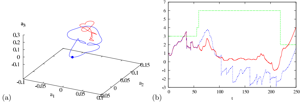
FIGURE 6. (a) Every slice hyperplane cuts every group orbit at least twice (see figure 5). An SO(2) relative periodic orbit is topologically a torus, so the two cuts are the two periodic orbit images of the same relative periodic orbit, the good close one, and the bad distant one, on the other side of slice border, and thus not in the slice. Here this is illustrated by close cut (blue, solid line) of the relative periodic orbit RPO_{36.72} torus, figure 1(b), plotted together with the most distant cut (red, dashed), in the same slice hyperplane, but not in the slice. (b) Comparison of symmetry-reduced trajectory using a single template ML (blue, short-dash) with the same trajectory symmetry reduced using the travelling waves in table 1 as template (red, solid) indexed by j(t) ( j = 1 laminar; 2 LB; 3 ML; 4 MU; 5 UB; 6 S2U; 7 S2L), with template at time t indicated on left ordinate by (green, long-dash) line. Right ordinate: the shift deviation from the mean shift, \ell(t) - \bar{c}t , where \bar{c} \simeq 1.274 is estimated by a long-time simulation. Both symmetry reductions begin with the same template and experience the same jumps in the shift starting at t \approx 40 . By starting to switch the templates at t \approx 60 , further jumps (seen for the blue, short-dash line) are avoided (red, solid line).
