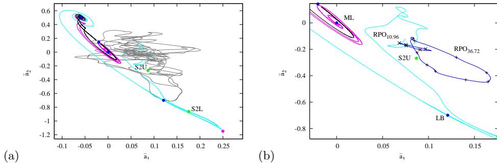
FIGURE 9. (a) Removal of the Z_2 symmetry of figure 8 opens the system to far more chaotic, or ‘turbulent’, transients (grey) within the S symmetry solution space that appear to frequently visit the travelling wave S2U, while the travelling wave S2L appears embedded into the laminar–turbulent boundary. The turbulent trajectory exhibits excursions to other states as well, most frequently ML and LB. (b) Two relative periodic orbits embedded within turbulence, the same symmetry-reduced state space projection as figure 8. Crosses are spaced every \Delta t = 2D/U on relative periodic orbit \text{RPO}_{10.96} and pluses are spaced 4D/U on relative periodic orbit \text{RPO}_{36.72} . On this scale the tiny \text{RPO}_{4.934} [figure 8 (b), inset] only explores a region about the size of the plot dots, and plays no role in turbulent dynamics.
